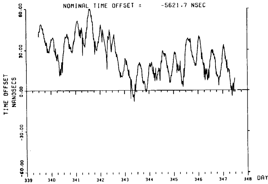
FIGURE 3. INTERFEROMETRIC TIME OFFSET CORRECTIONS FOR PRN3/NAV11 FOR WEEK 413
